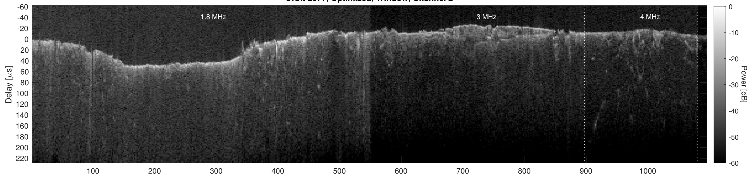
Orbit 2677, Cluttergram
