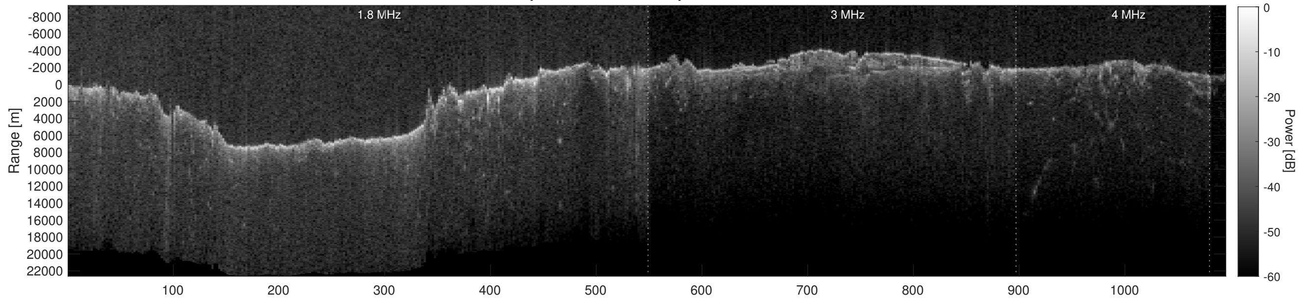
Orbit 2677, Depth-Corrected Cluttergram
