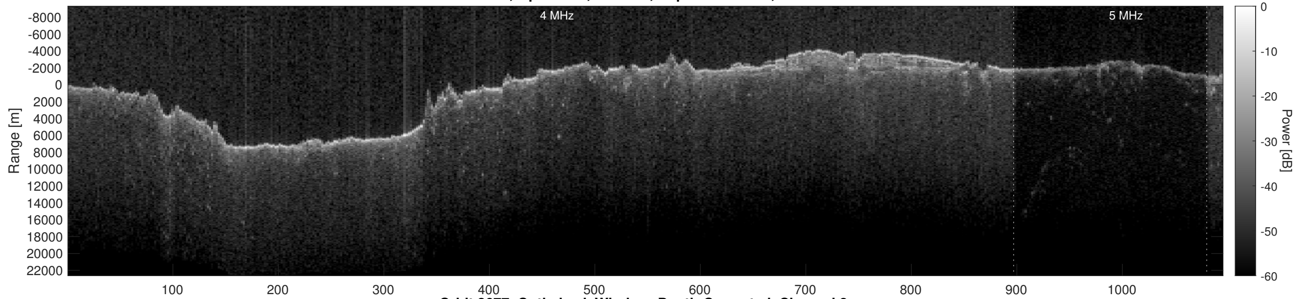
Orbit 2677, Optimized, Window, Depth-Corrected, Channel 2
