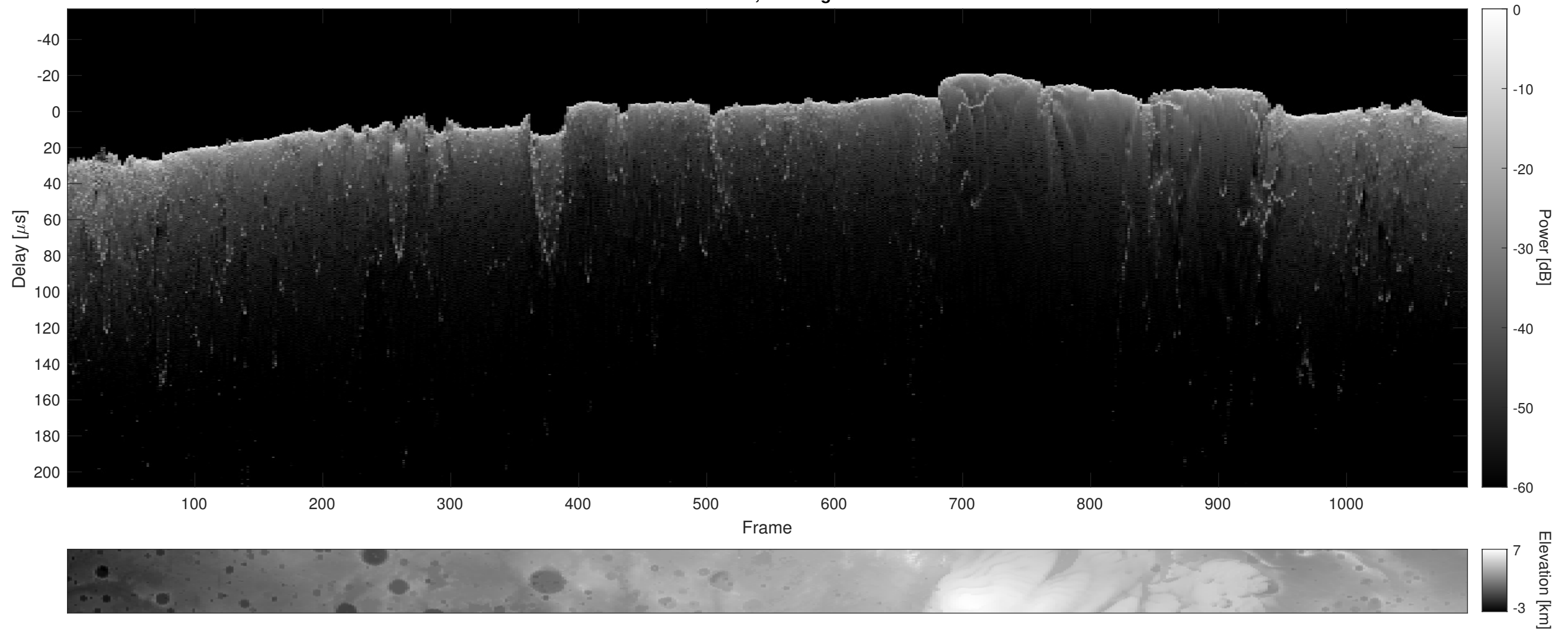
Orbit 2678, Cluttergram
