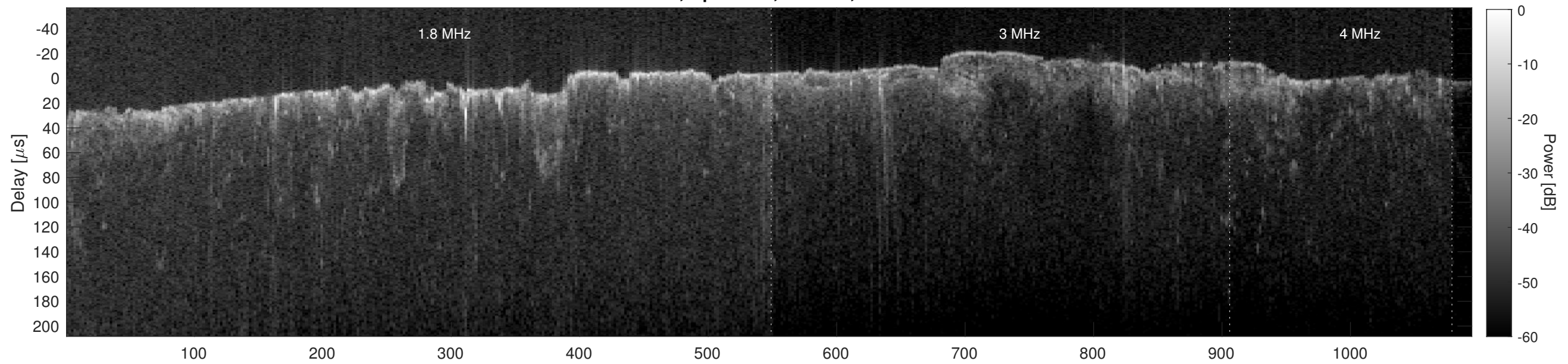
Orbit 2678, Cluttergram
