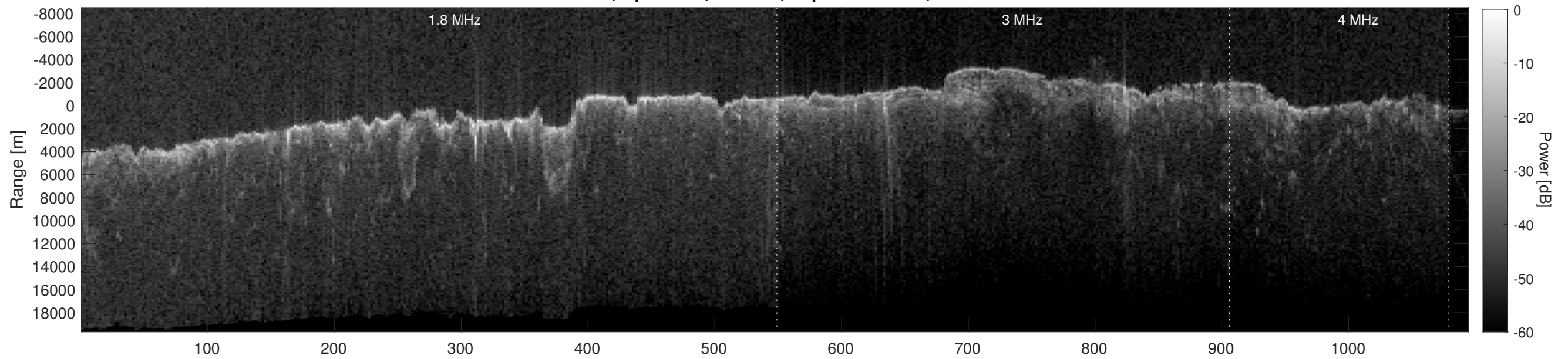
Orbit 2678, Depth-Corrected Cluttergram
