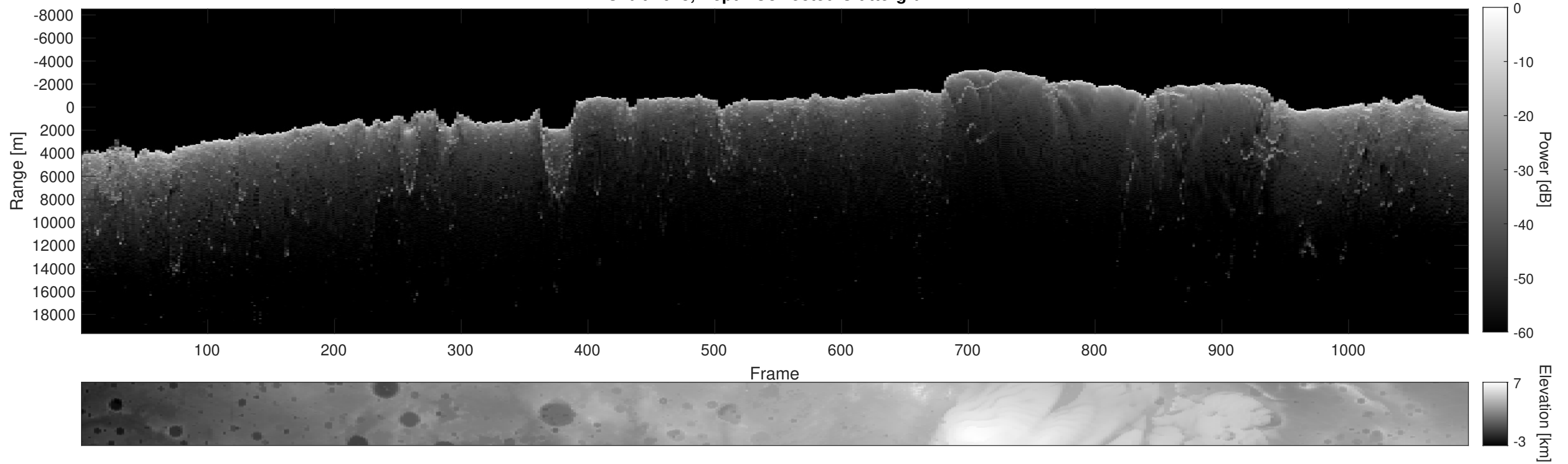
Orbit 2678, Depth-Corrected Cluttergram
