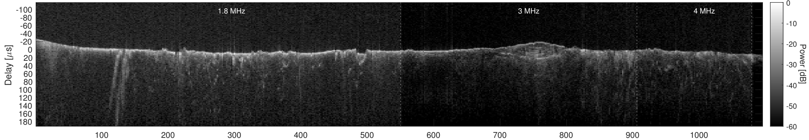
Orbit 2679, Cluttergram
