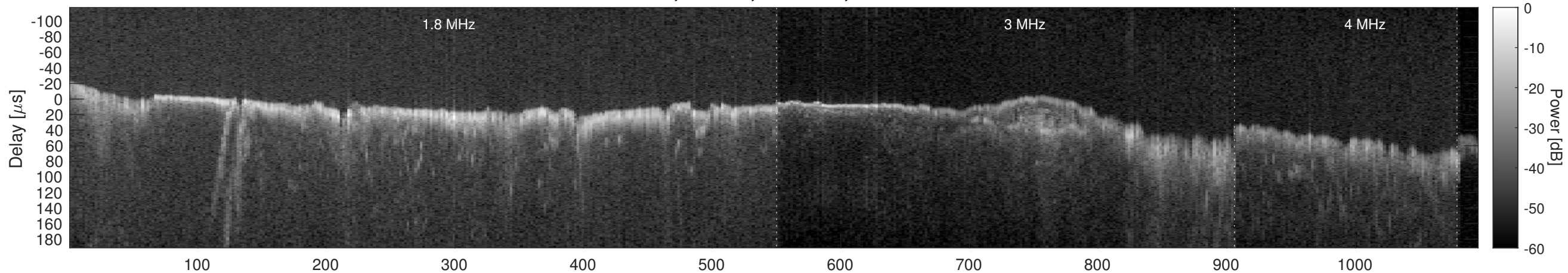
Orbit 2679, Window, Channel 2, Chapman
