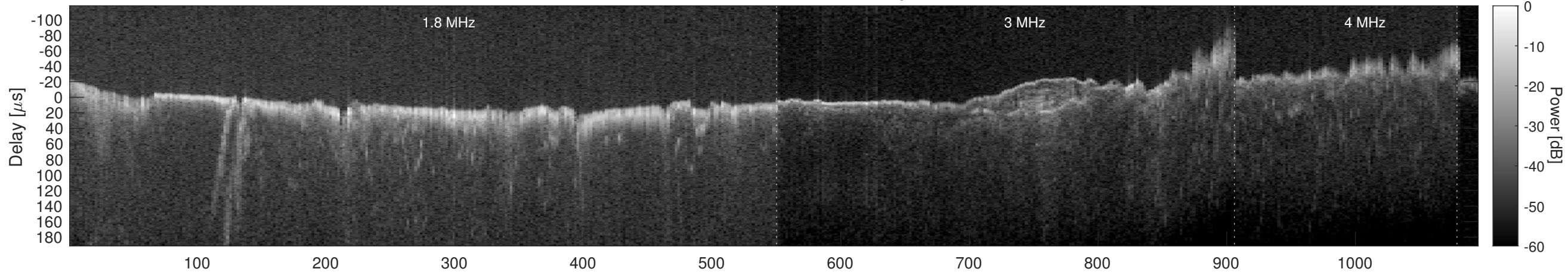
Orbit 2679, Window, Channel 2, Optimized
