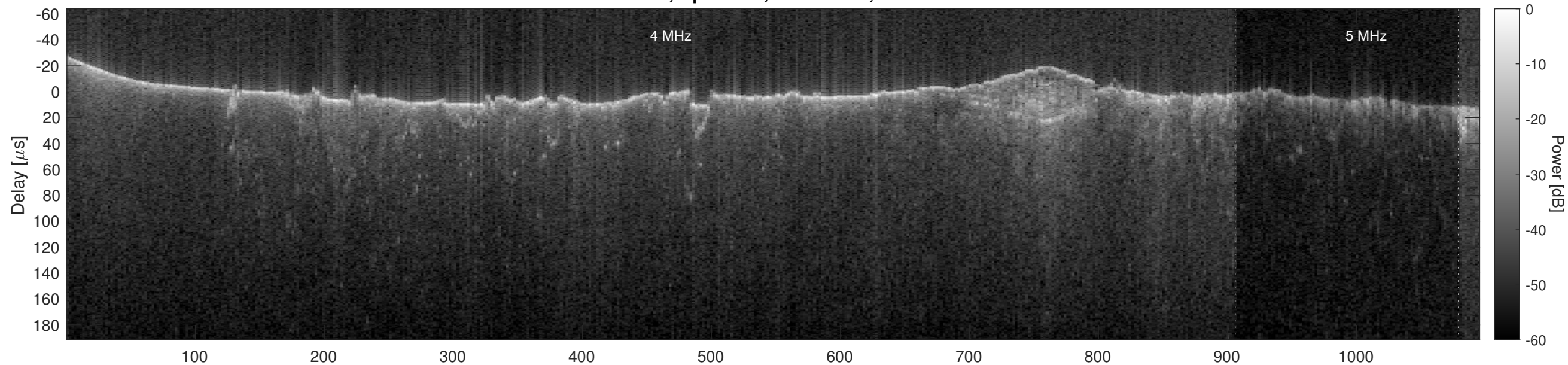
Orbit 2679, Optimized, No Window, Channel 2
