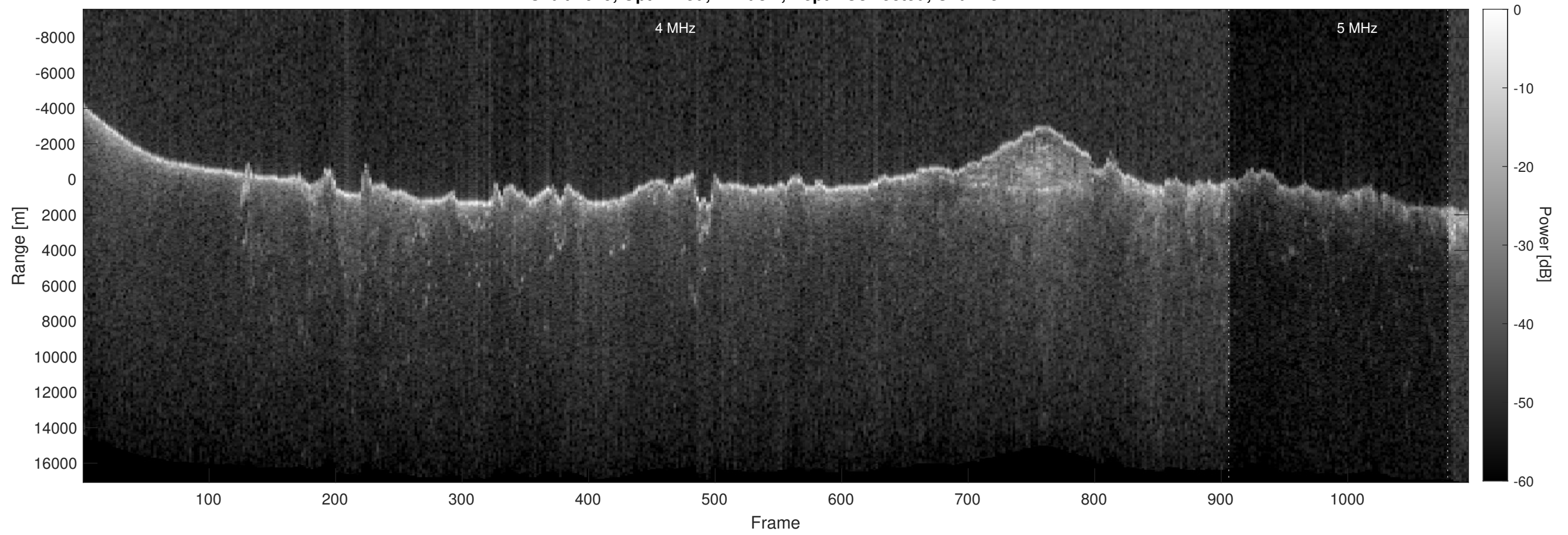
Orbit 2679, Optimized, Window, Depth-Corrected, Channel 2
