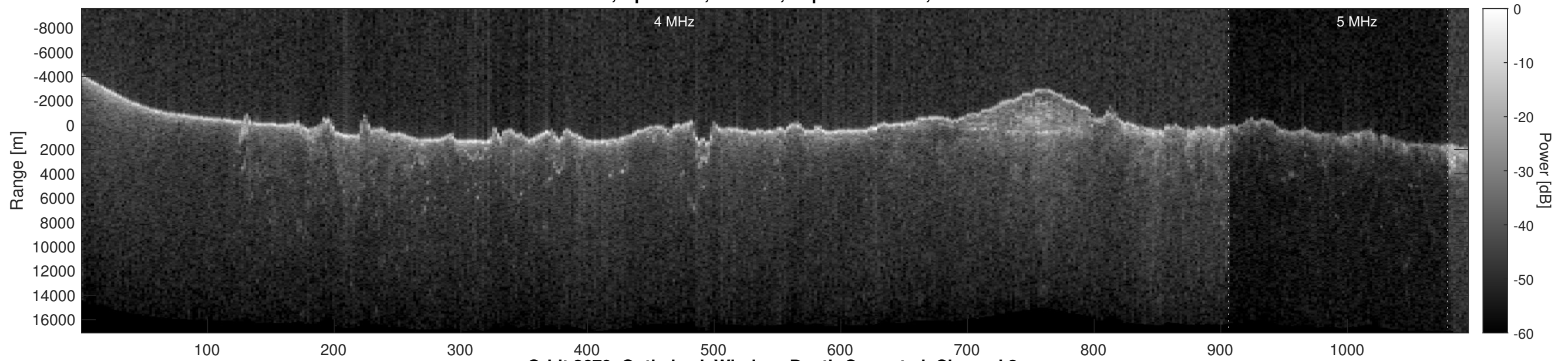
Orbit 2679, Optimized, Window, Depth-Corrected, Channel 2
