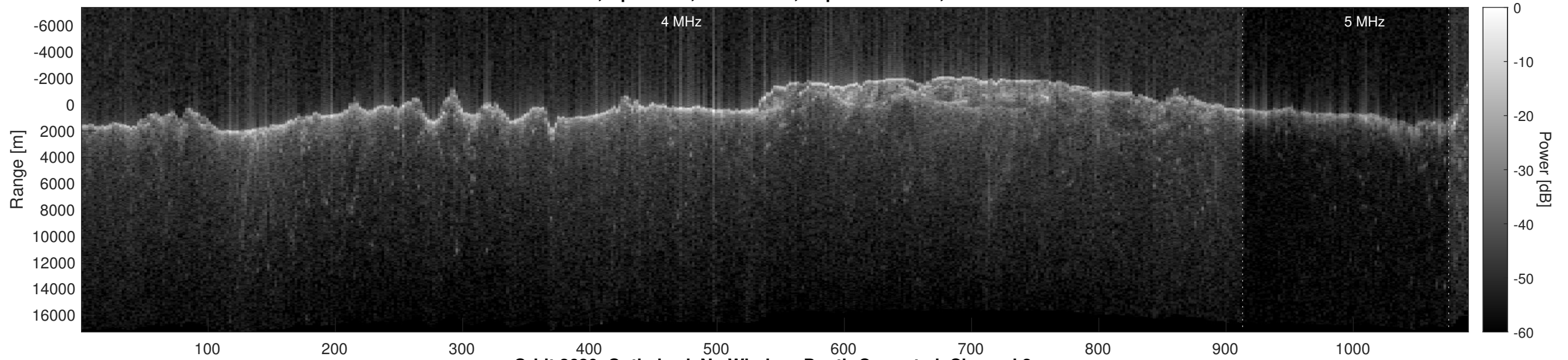
Orbit 2680, Optimized, No Window, Depth-Corrected, Channel 2
