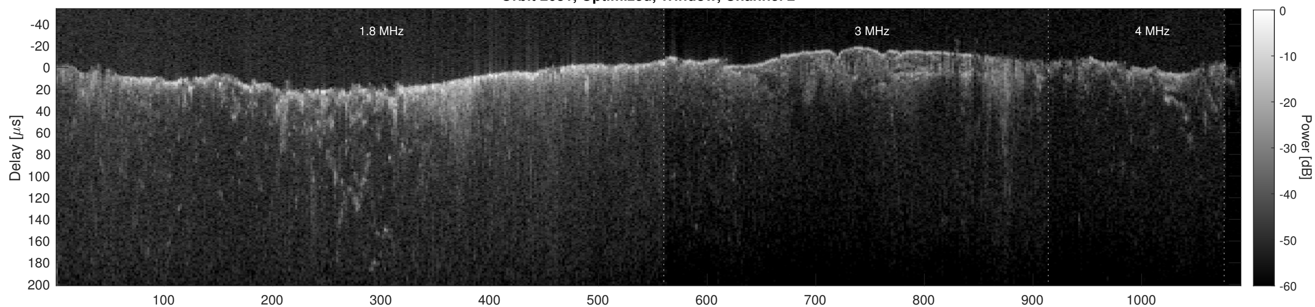
Orbit 2681, Cluttergram
