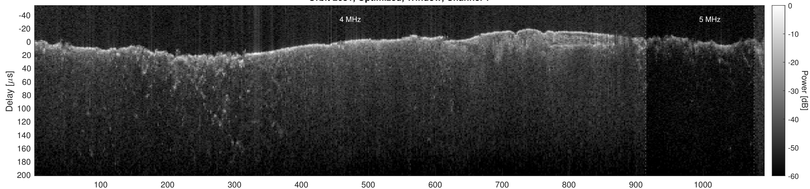
Orbit 2681, Optimized, Window, Channel 2
