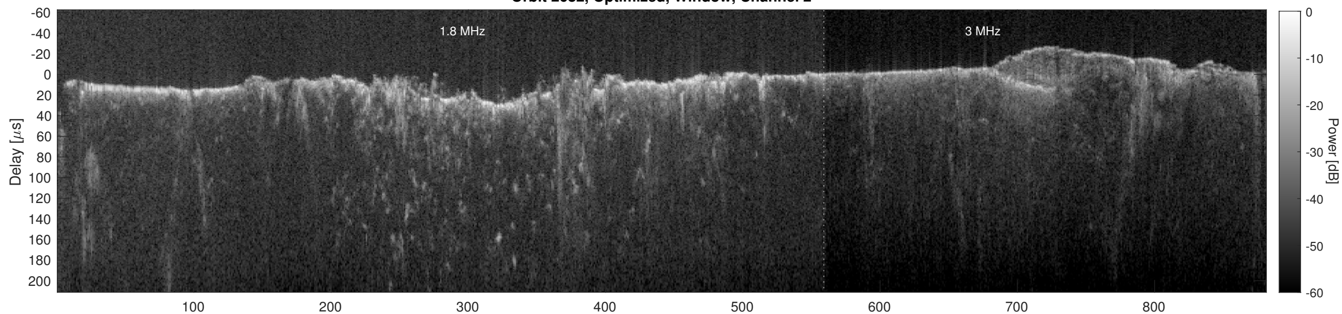
Orbit 2682, Cluttergram
