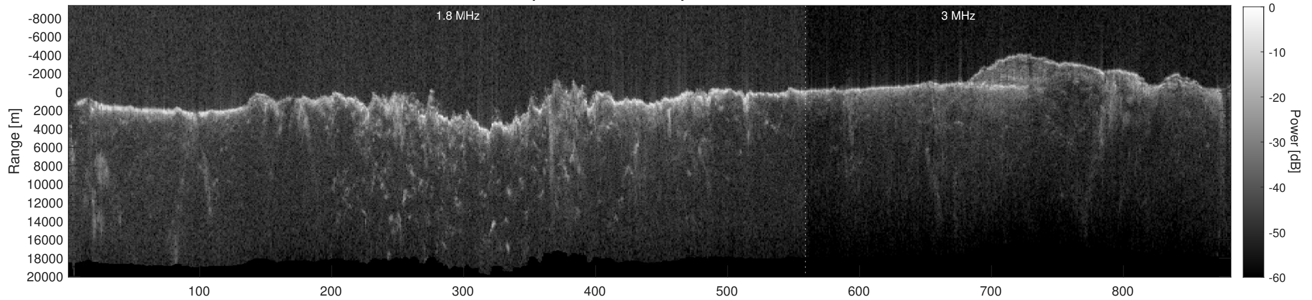
Orbit 2682, Depth-Corrected Cluttergram
