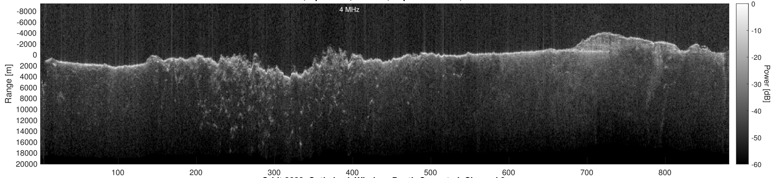
Orbit 2682, Optimized, Window, Depth-Corrected, Channel 2
