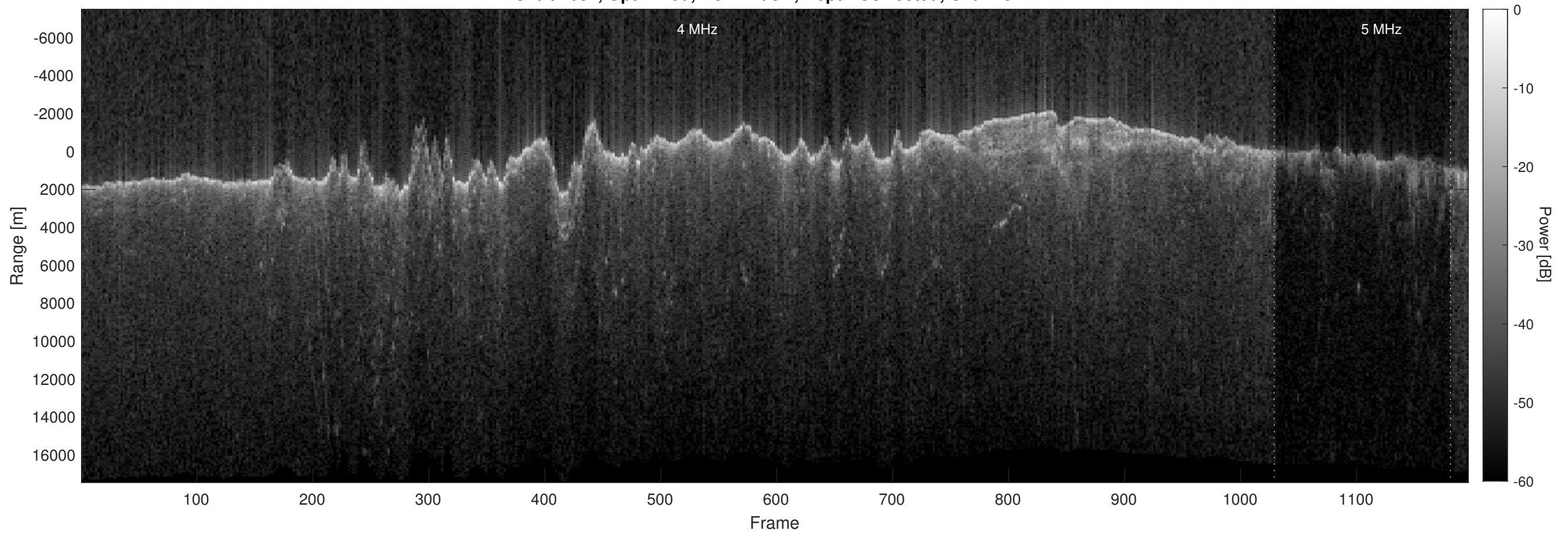
Orbit 2684, Optimized, No Window, Depth-Corrected, Channel 2
