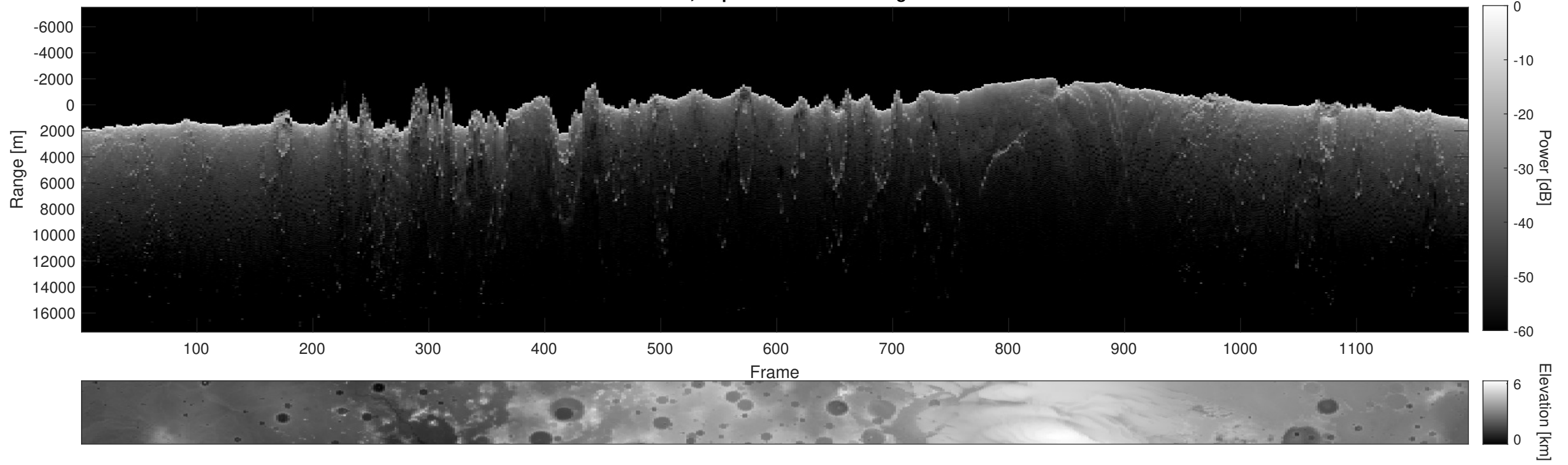
Orbit 2684, Depth-Corrected Cluttergram
