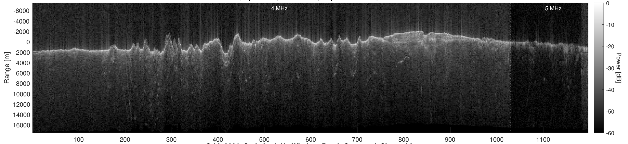
Orbit 2684, Optimized, No Window, Depth-Corrected, Channel 2
