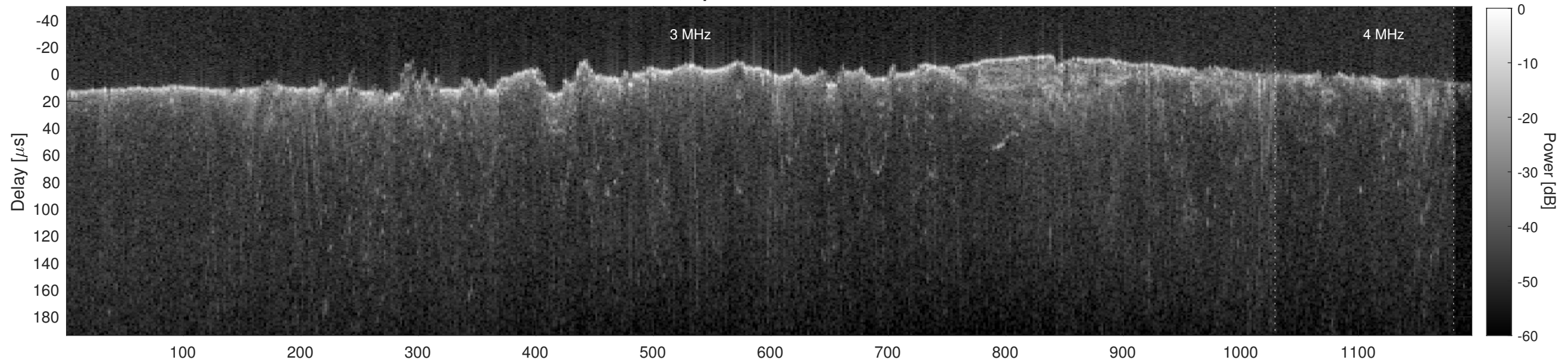
Orbit 2684, Cluttergram
