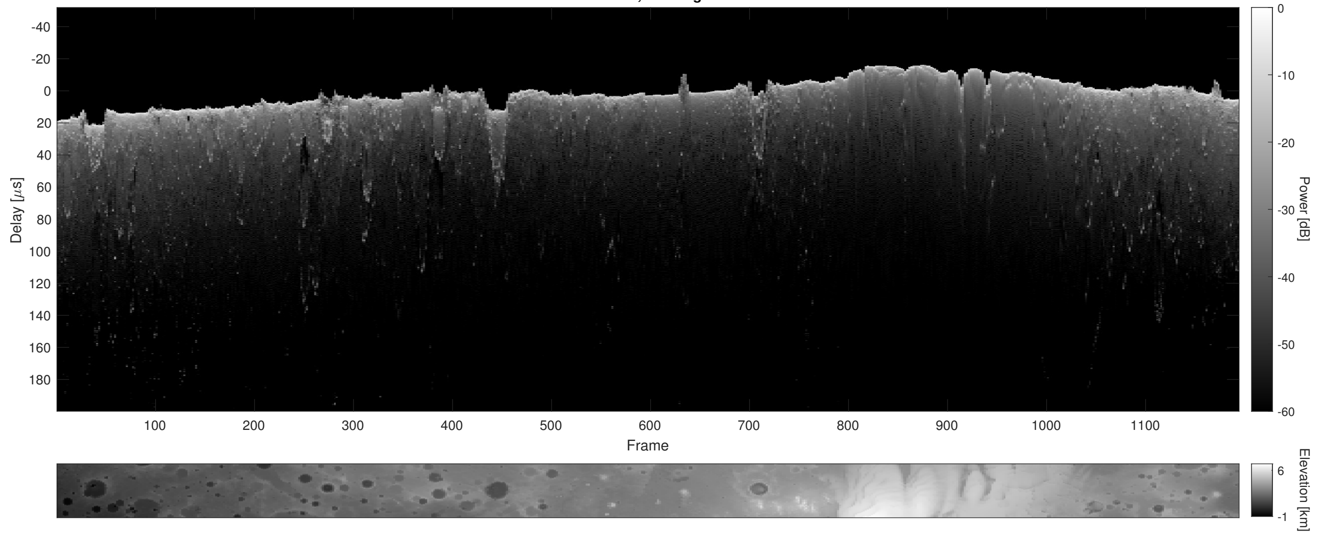
Orbit 2685, Cluttergram
