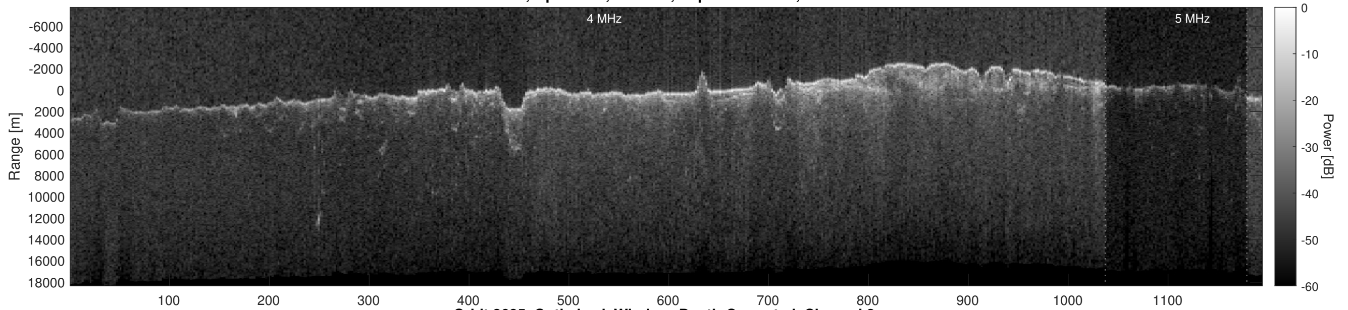
Orbit 2685, Optimized, Window, Depth-Corrected, Channel 2
