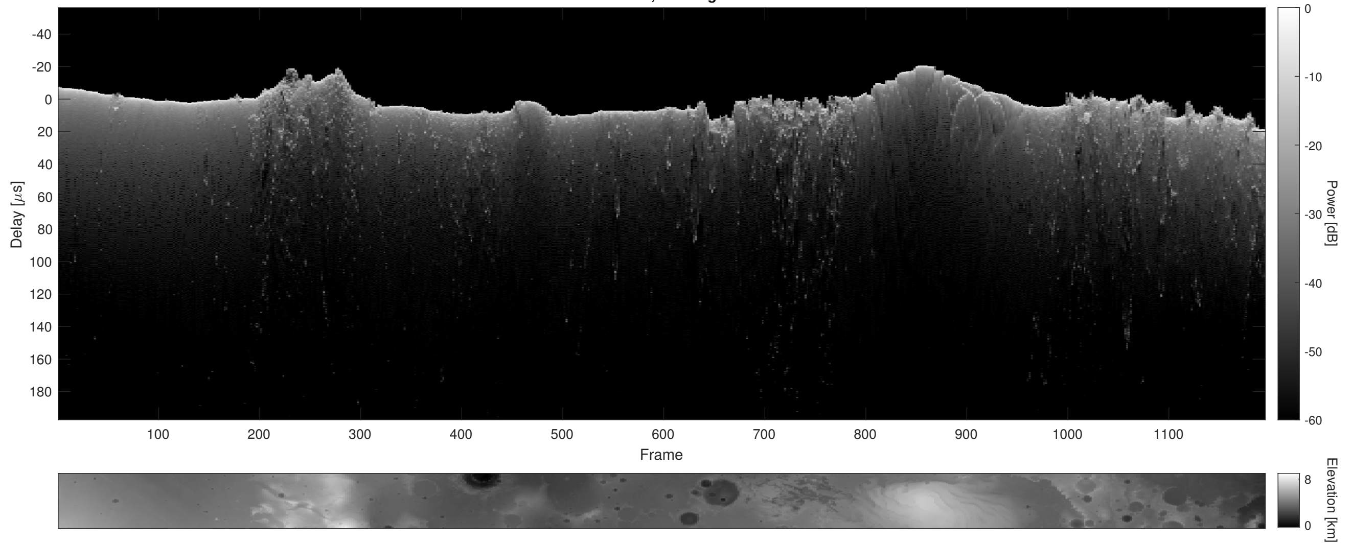
Orbit 2686, Cluttergram
