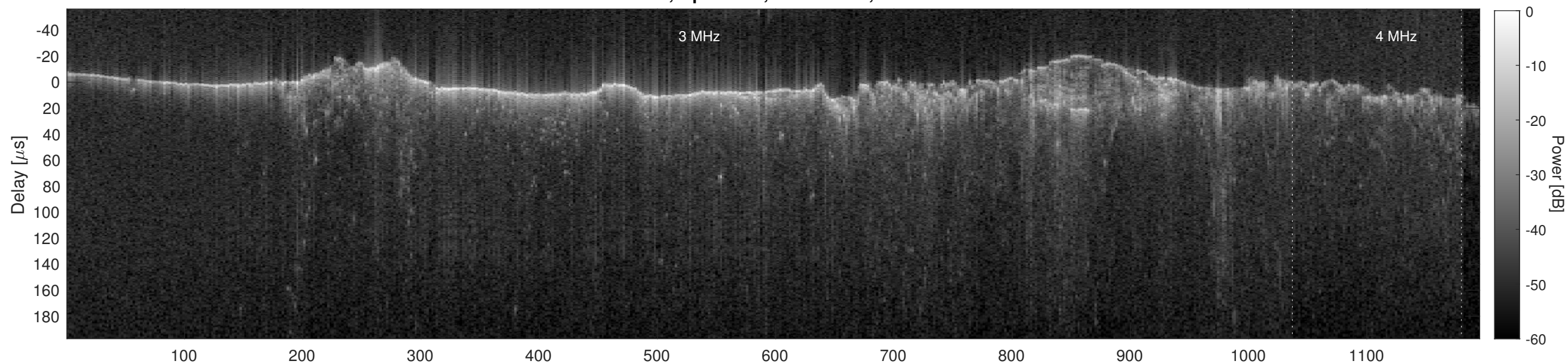
Orbit 2686, Cluttergram
