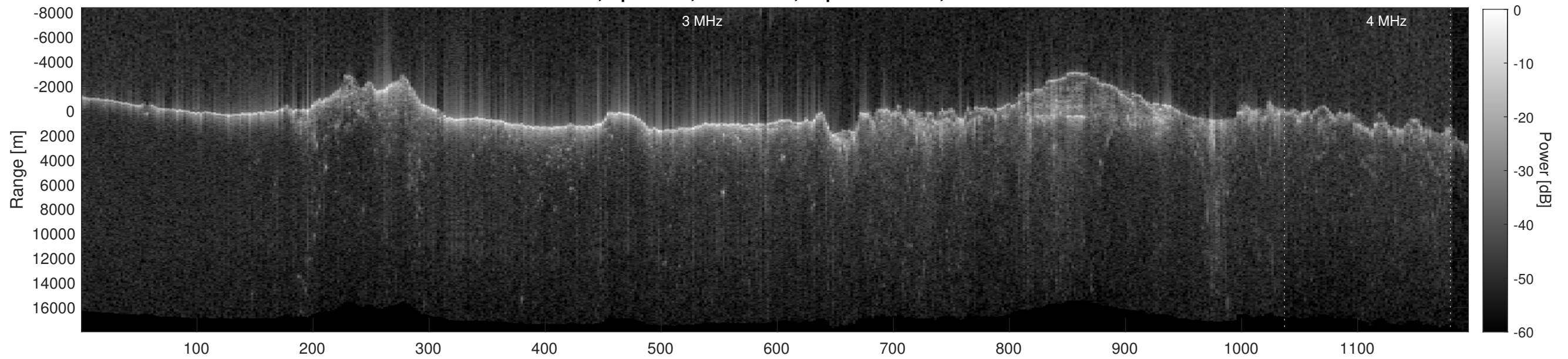
Orbit 2686, Depth-Corrected Cluttergram
