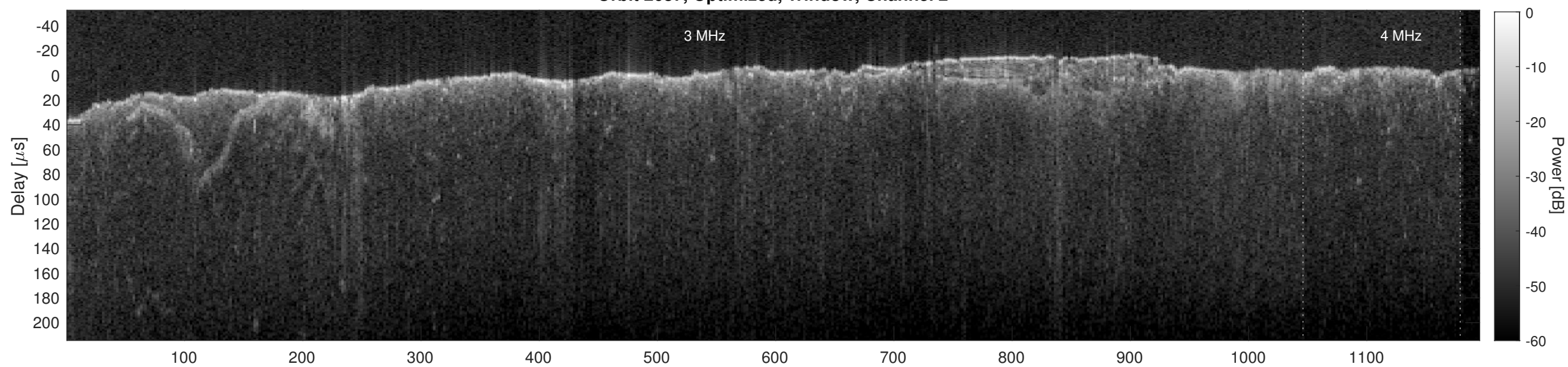
Orbit 2687, Cluttergram
