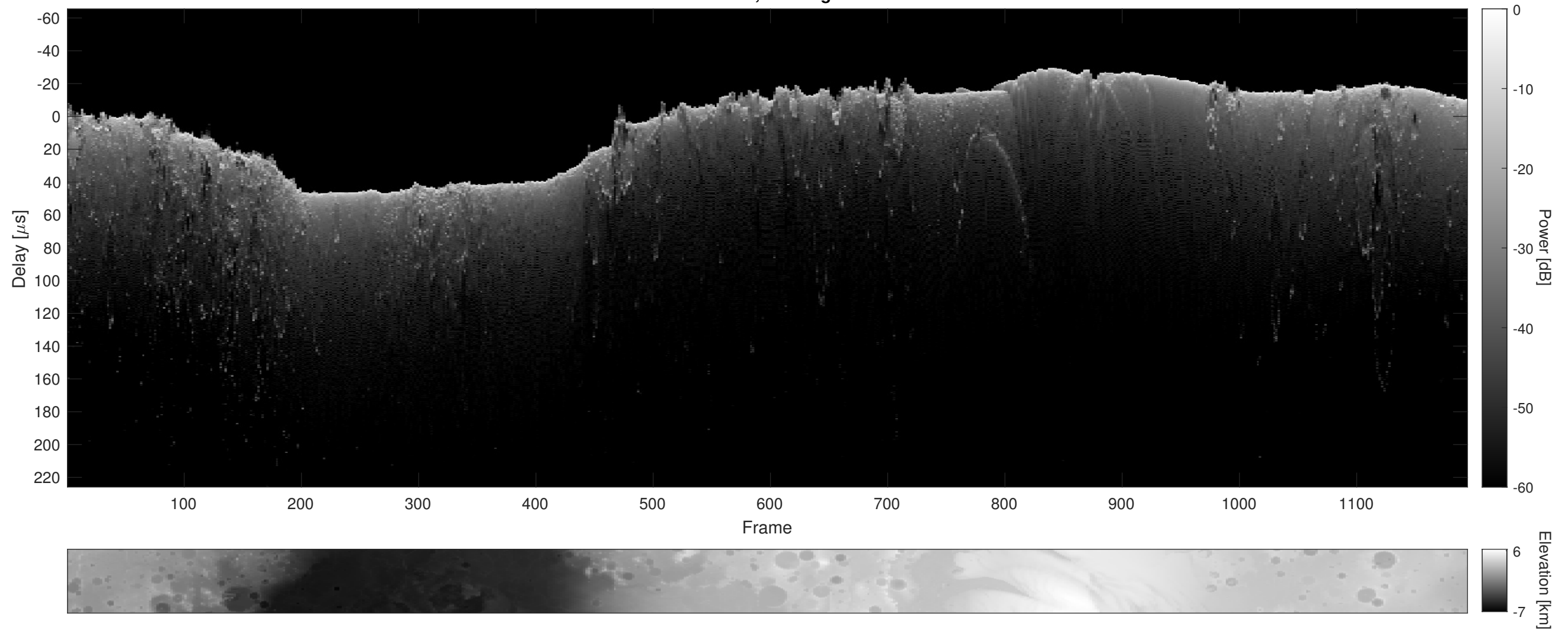
Orbit 2688, Cluttergram
