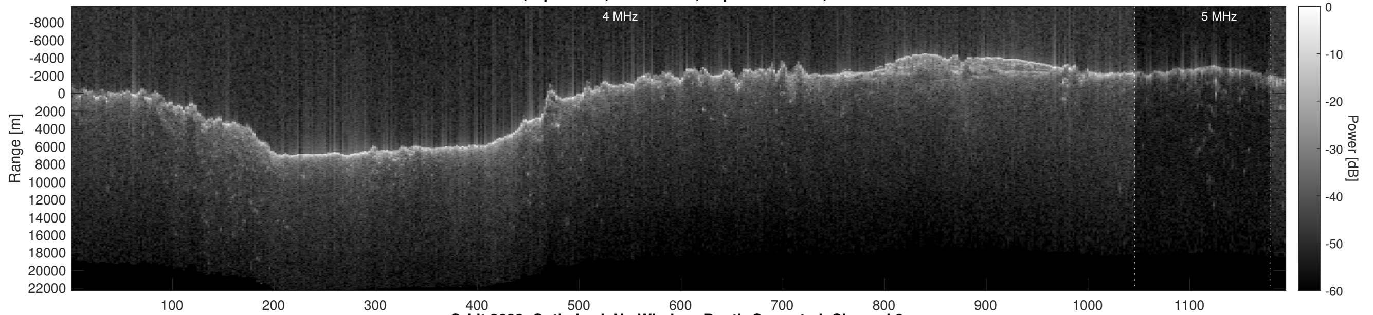
Orbit 2688, Optimized, No Window, Depth-Corrected, Channel 2
