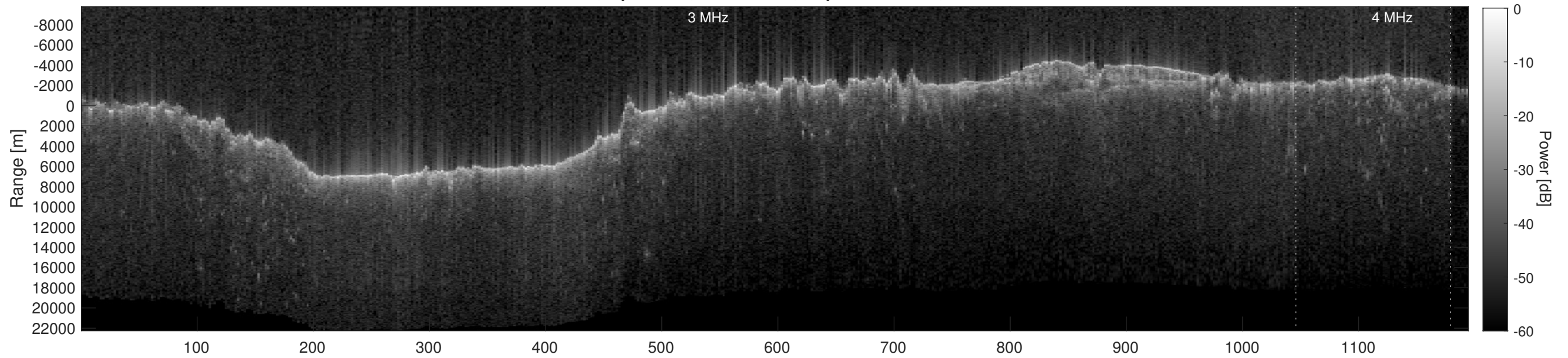
Orbit 2688, Depth-Corrected Cluttergram
