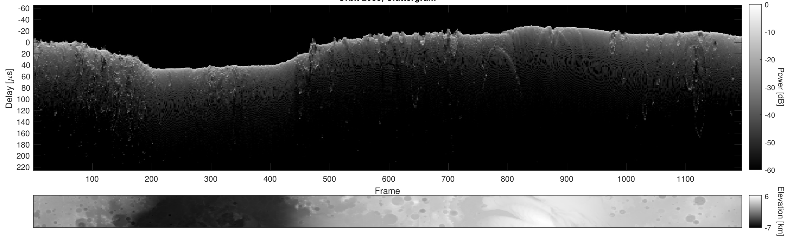
Orbit 2688, Cluttergram
