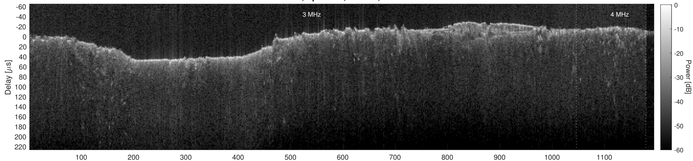
Orbit 2688, Cluttergram
