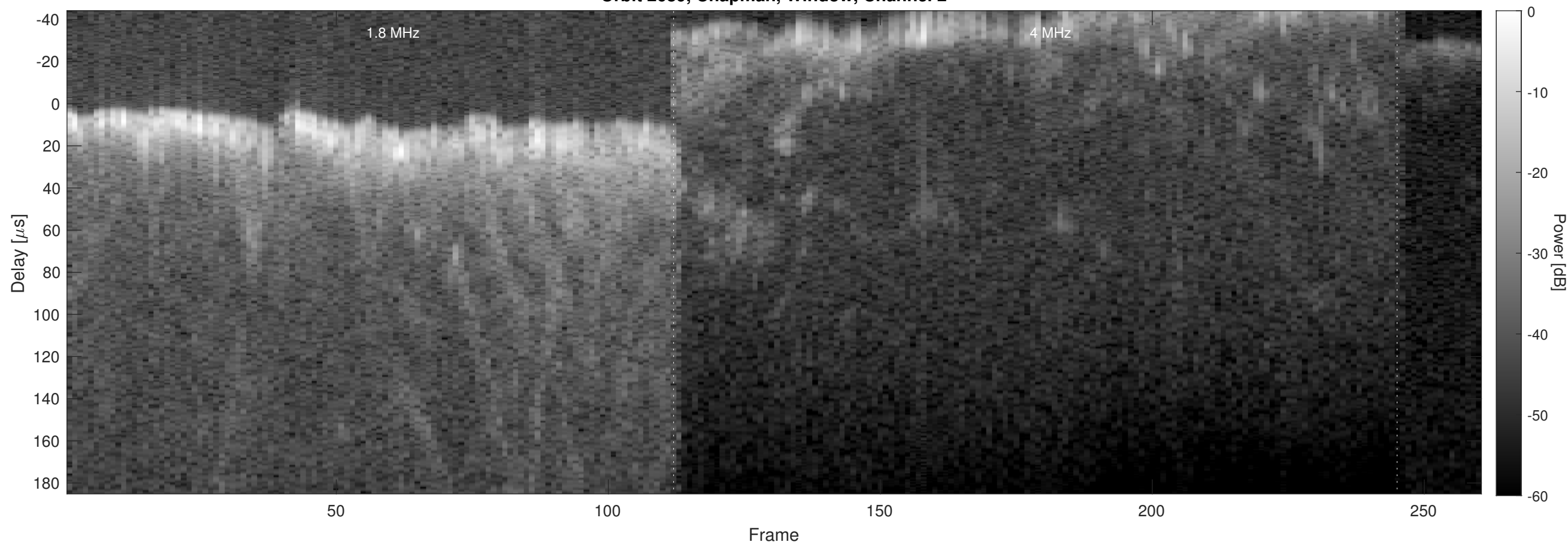
Orbit 2689, Chapman, Window, Channel 2
