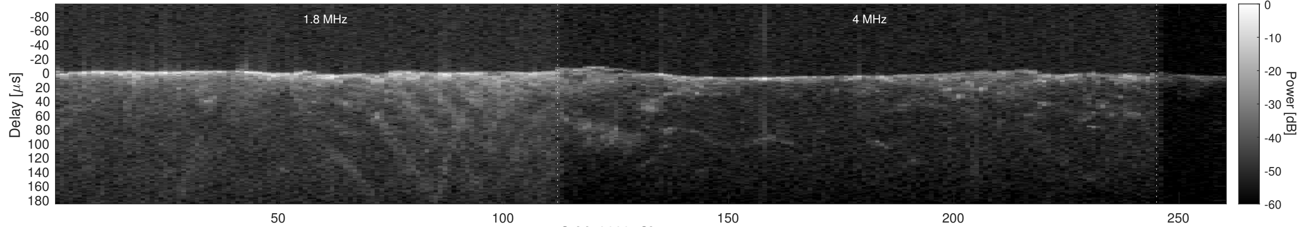
Orbit 2689, Cluttergram
