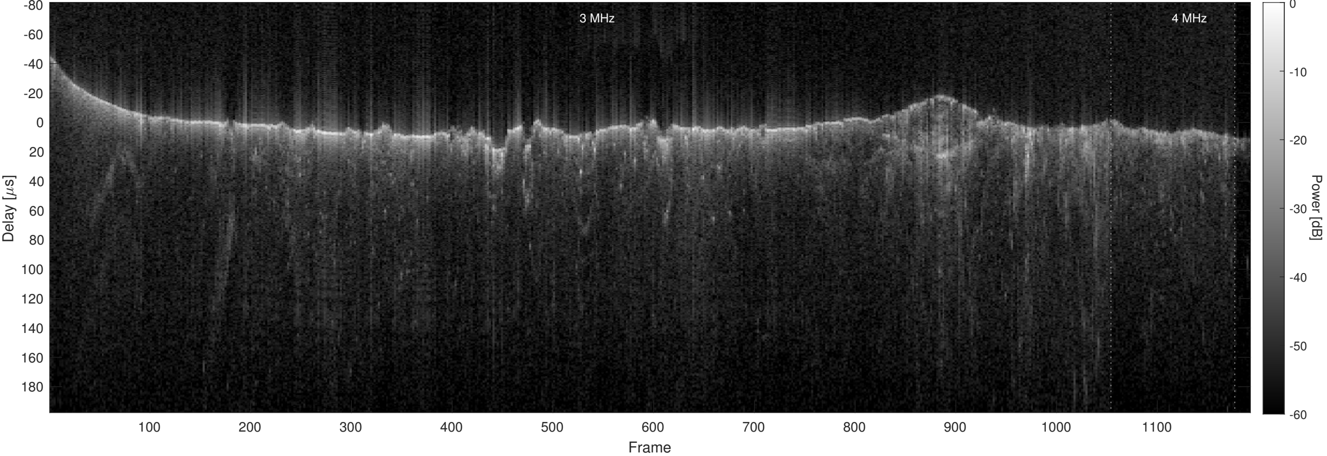
Orbit 2690, Optimized, No Window, Channel 2
