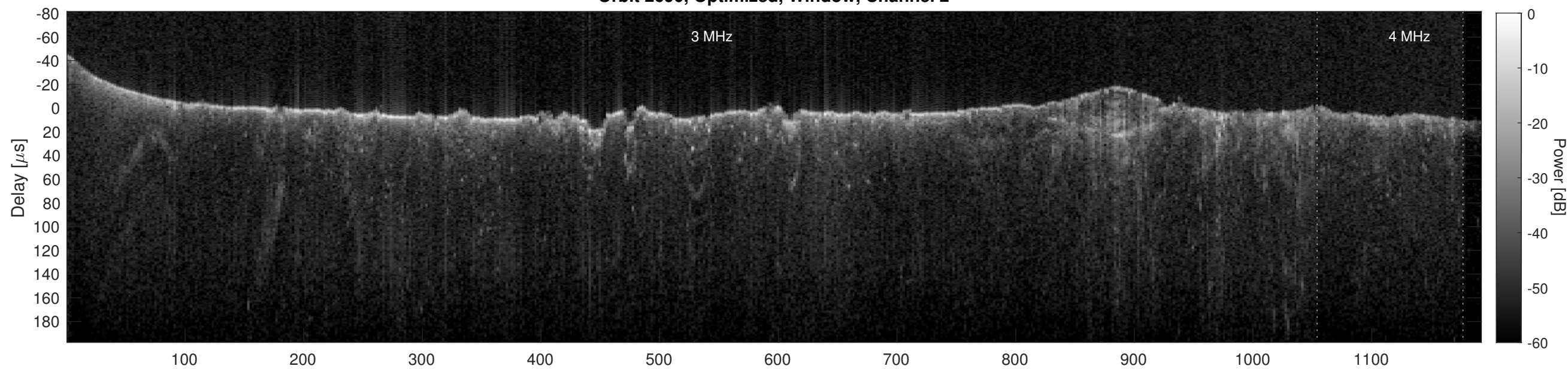
Orbit 2690, Cluttergram
