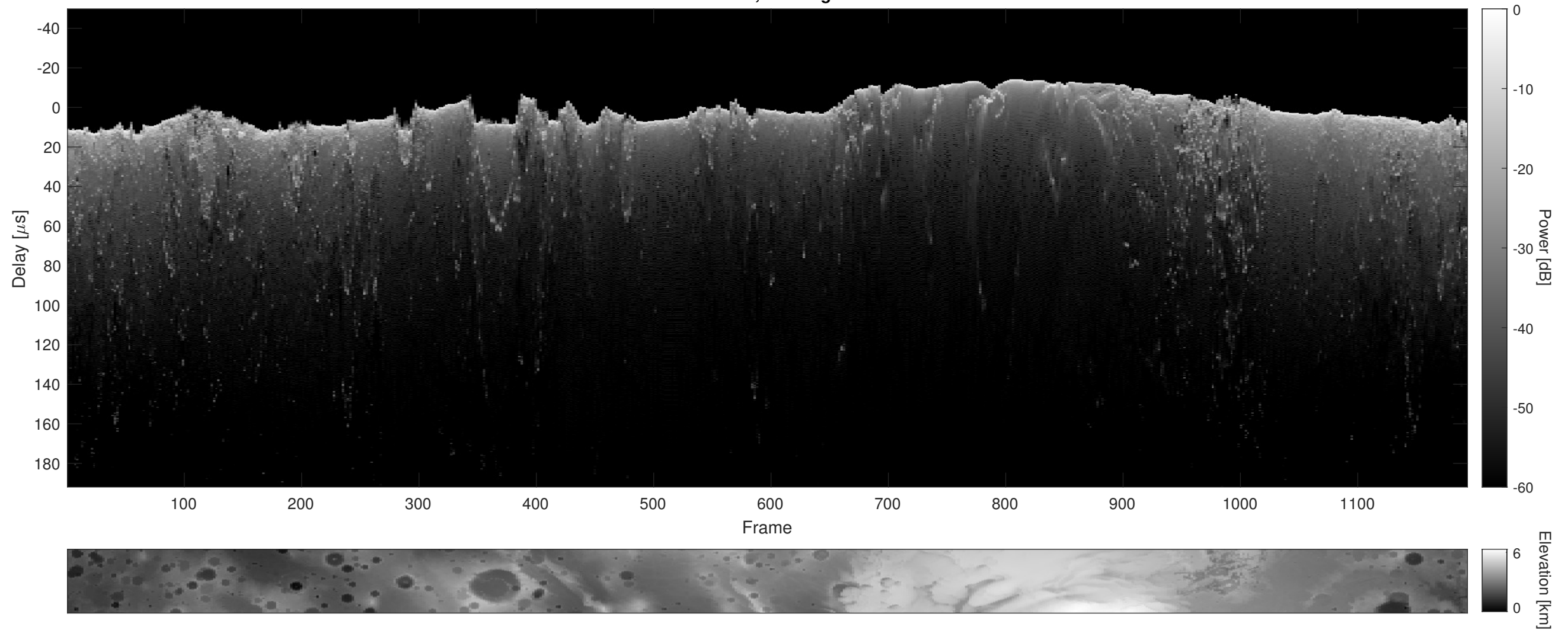
Orbit 2691, Cluttergram
