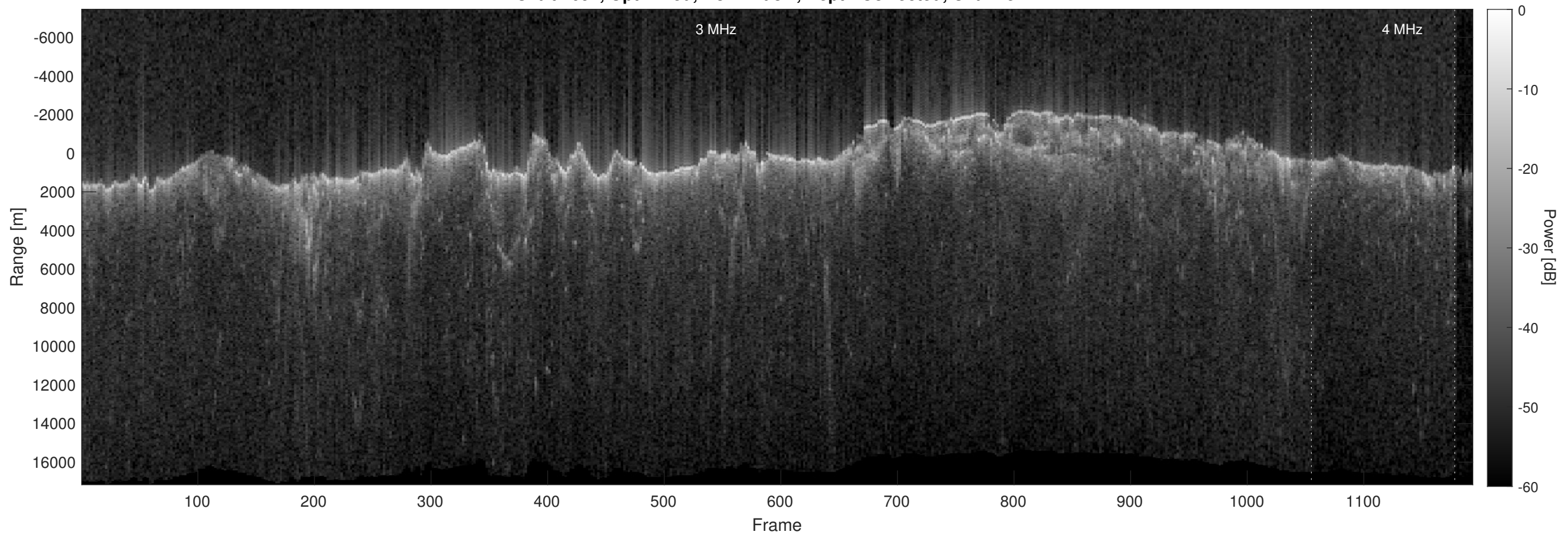
Orbit 2691, Optimized, No Window, Depth-Corrected, Channel 2
