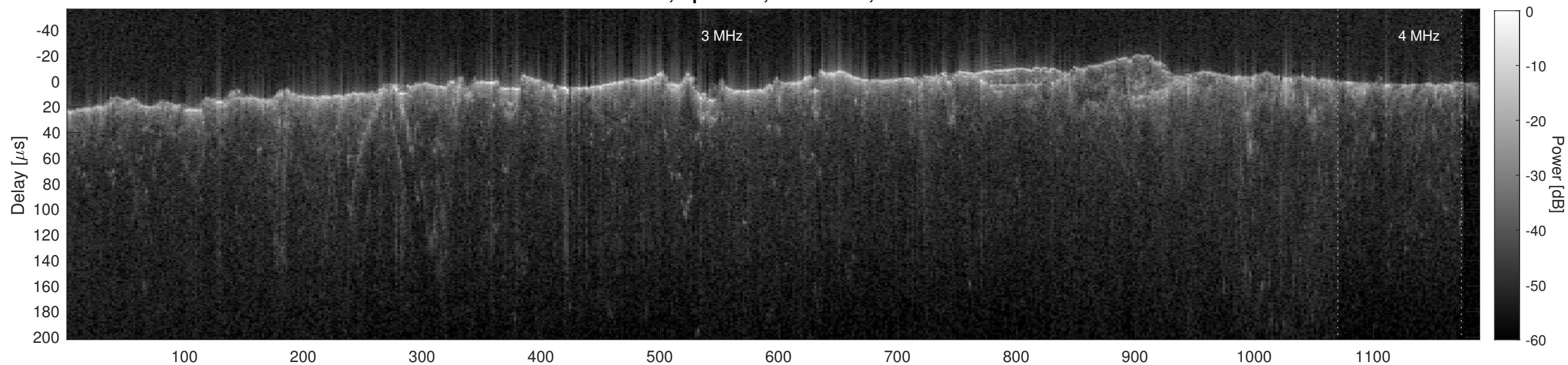
Orbit 2694, Cluttergram
