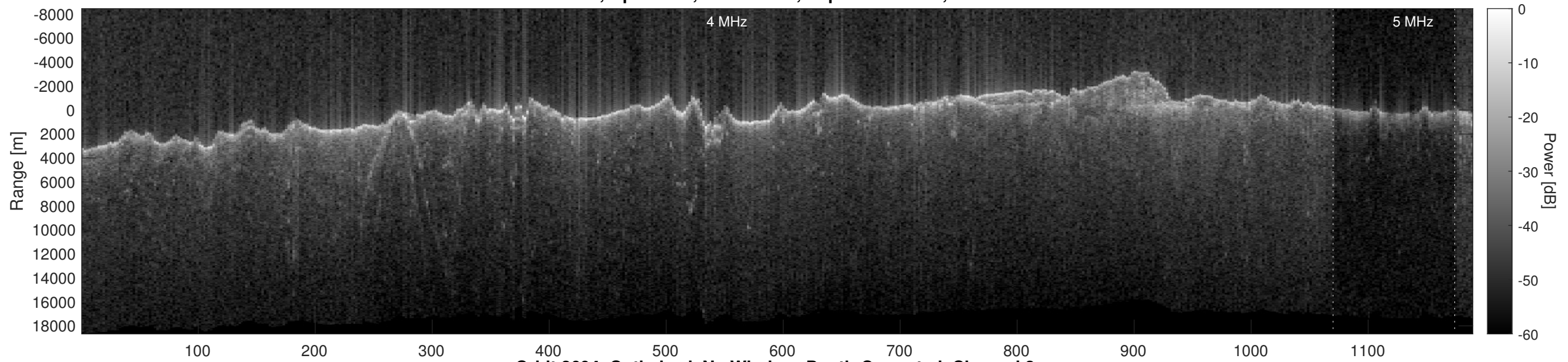
Orbit 2694, Optimized, No Window, Depth-Corrected, Channel 2
