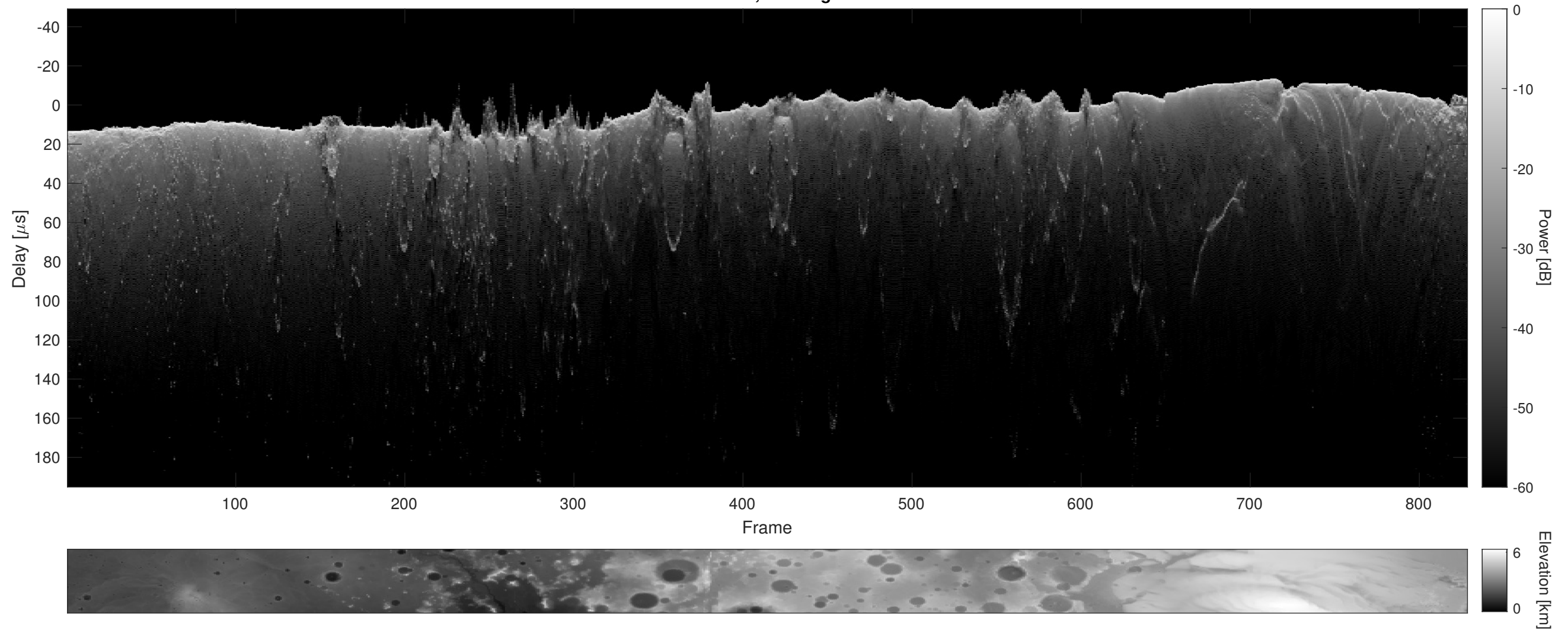
Orbit 2695, Cluttergram
