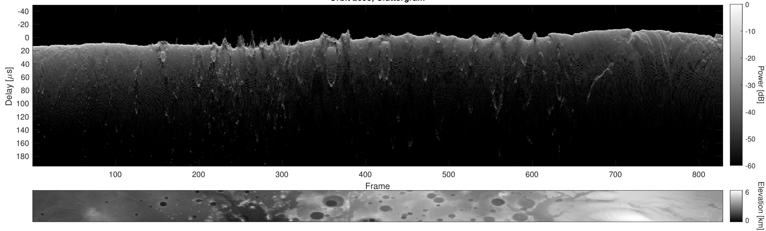
Orbit 2695, Cluttergram
