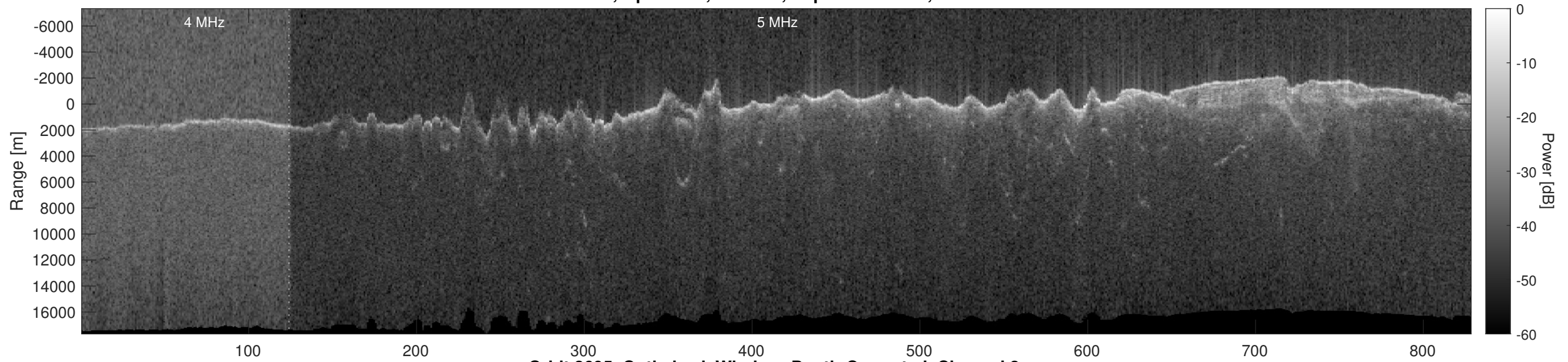
Orbit 2695, Optimized, Window, Depth-Corrected, Channel 2
