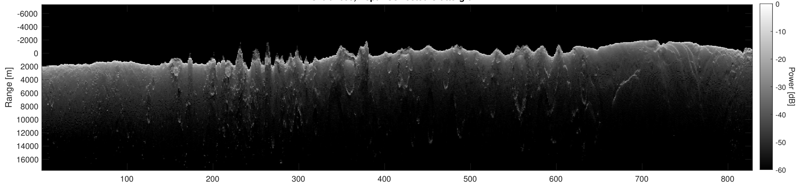
Orbit 2695, Depth-Corrected Cluttergram
