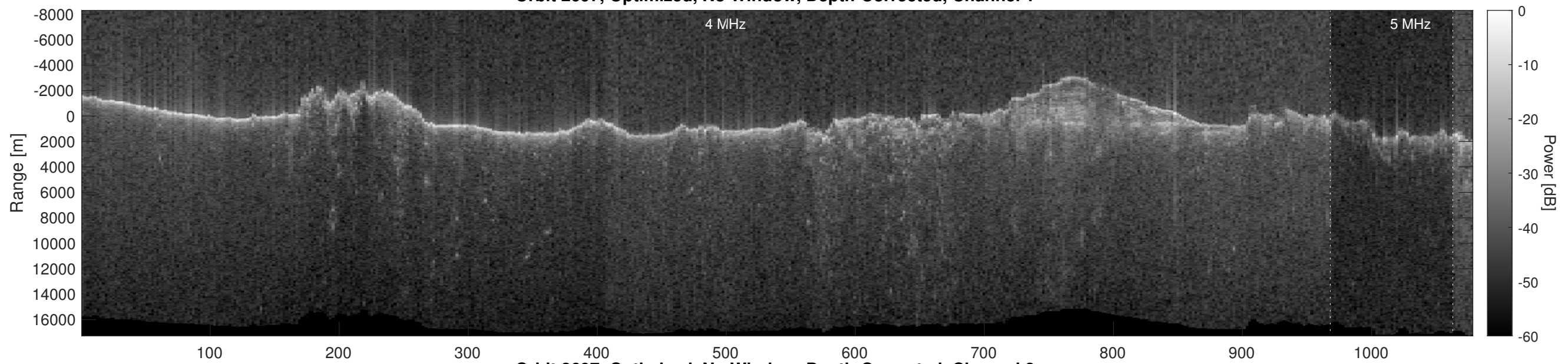
Orbit 2697, Optimized, No Window, Depth-Corrected, Channel 2
