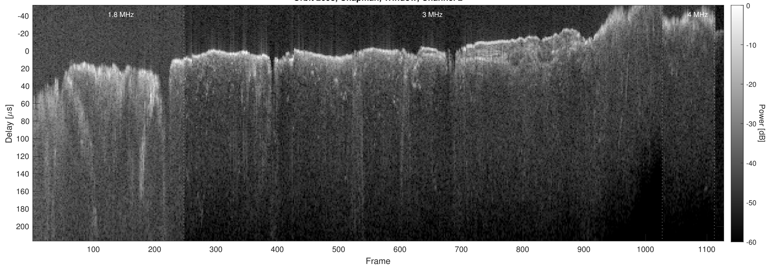
Orbit 2698, Chapman, Window, Channel 2
