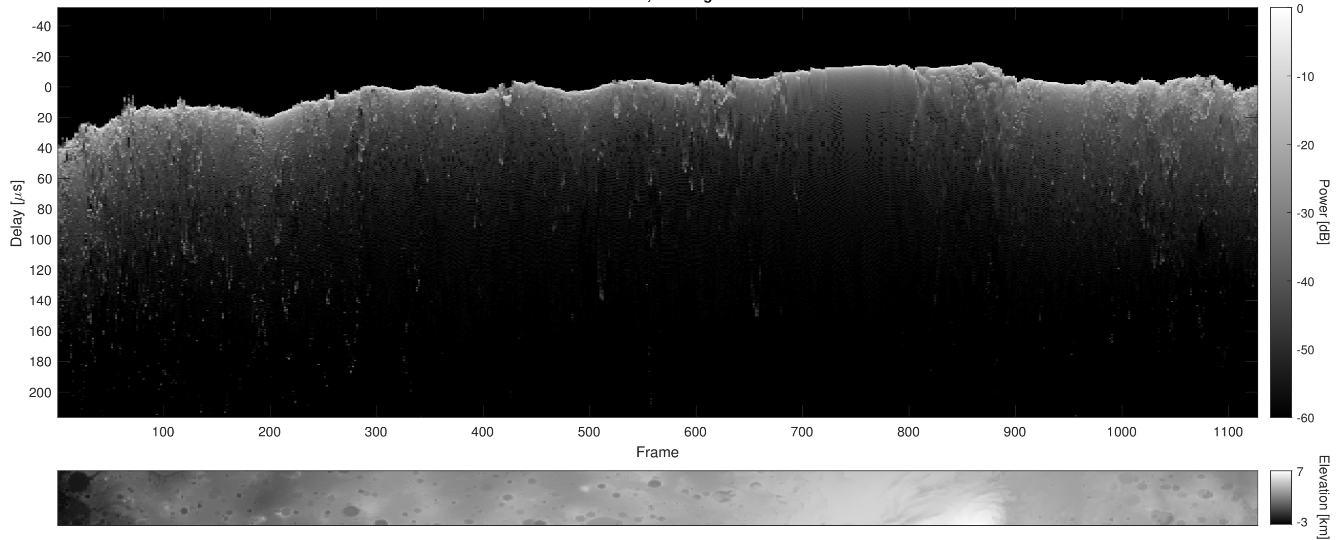
Orbit 2698, Cluttergram
