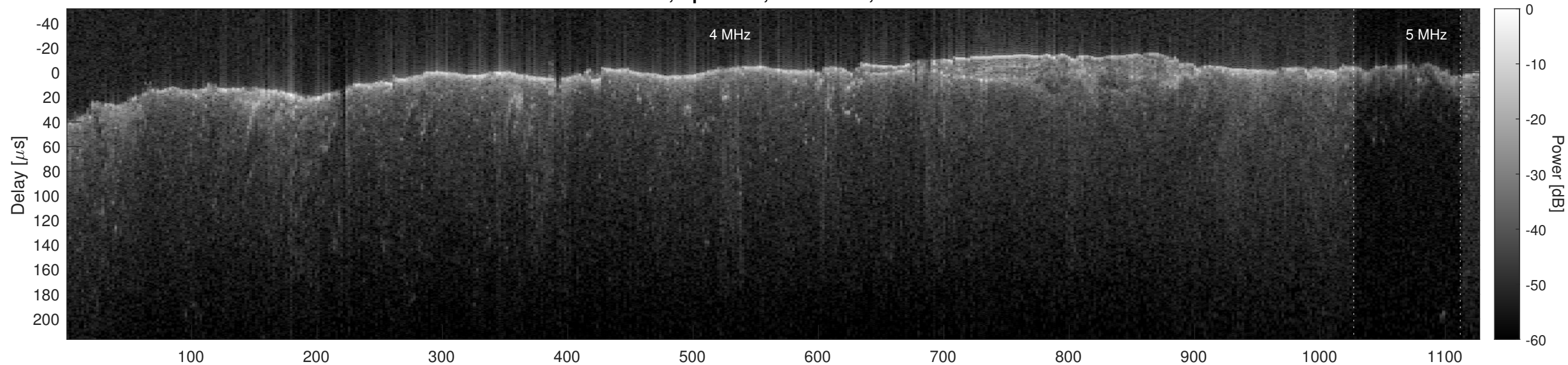
Orbit 2698, Optimized, No Window, Channel 2
