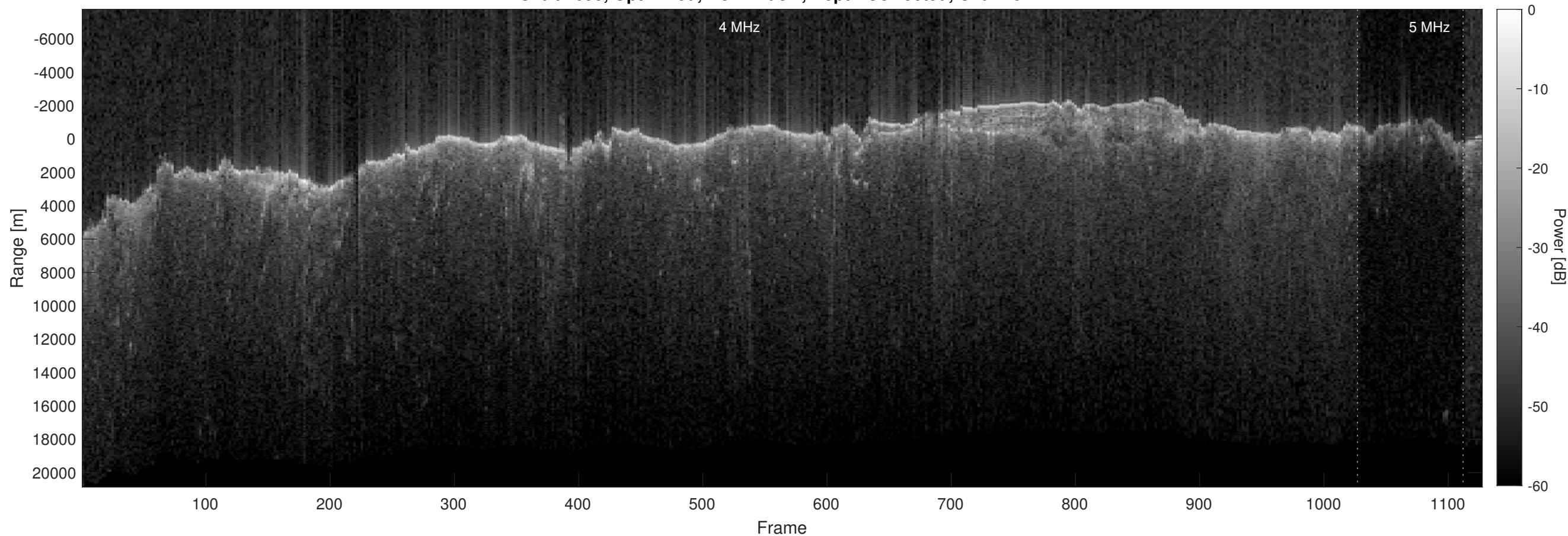
Orbit 2698, Optimized, No Window, Depth-Corrected, Channel 2
