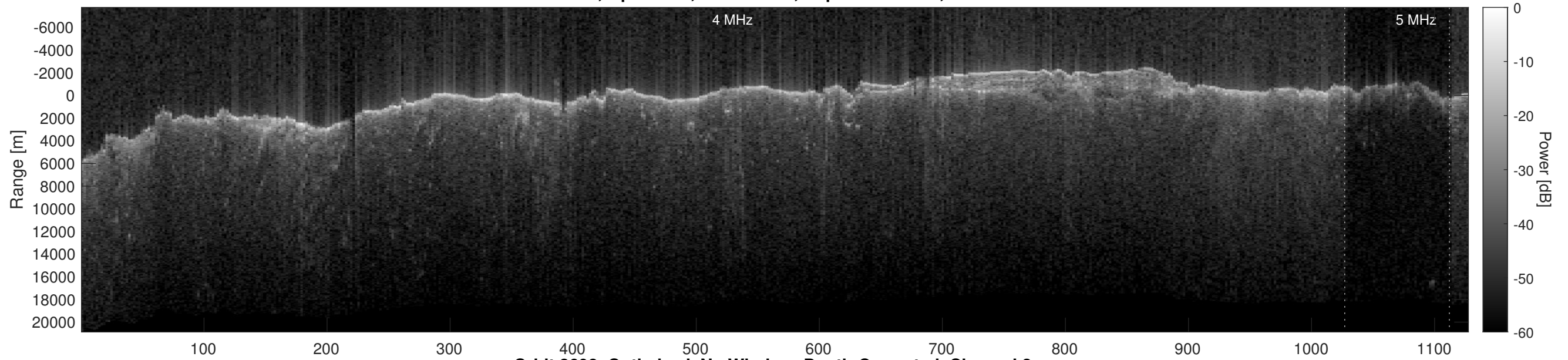
Orbit 2698, Optimized, No Window, Depth-Corrected, Channel 2
