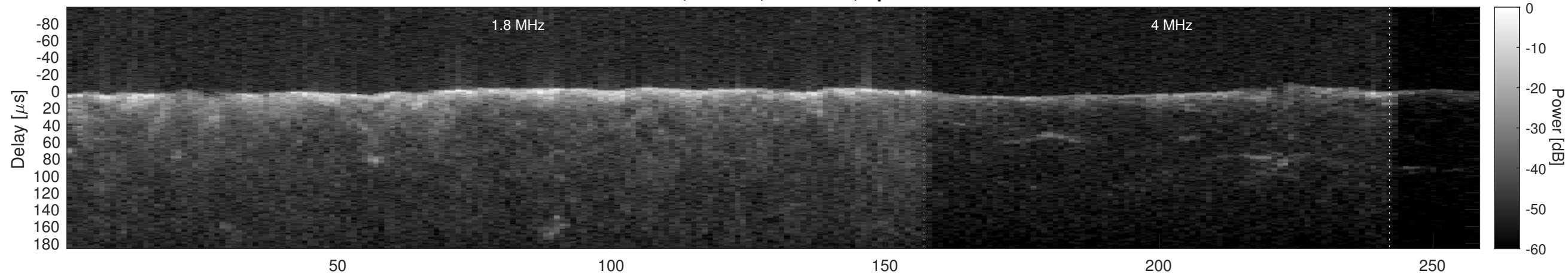
Orbit 2700, Cluttergram
