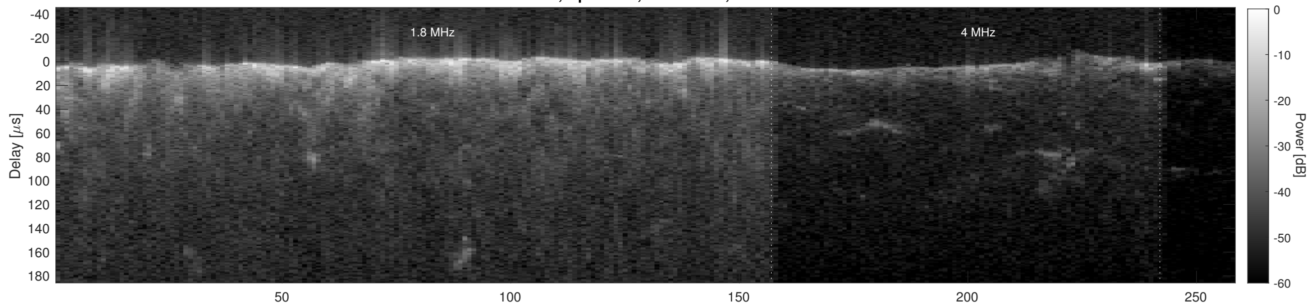
Orbit 2700, Cluttergram
