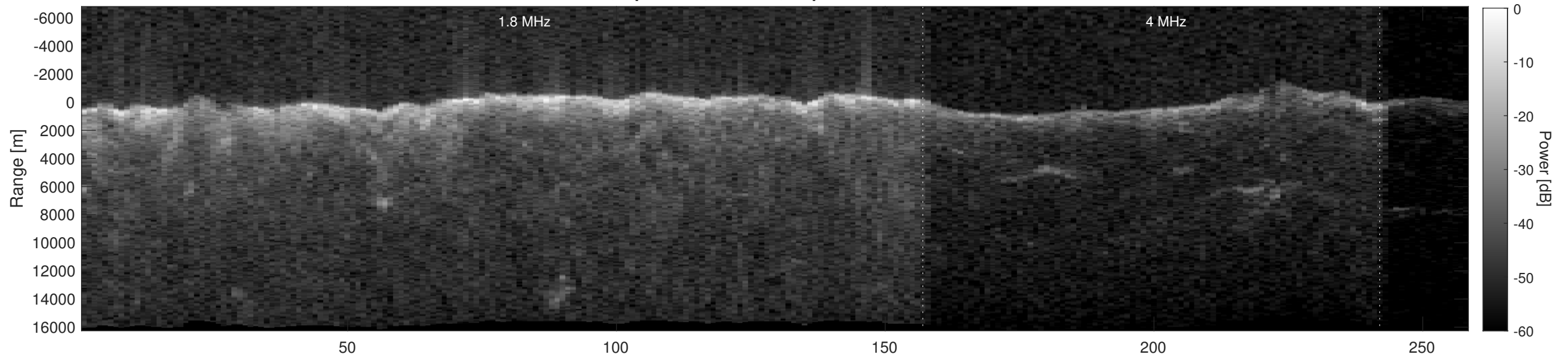
Orbit 2700, Depth-Corrected Cluttergram
