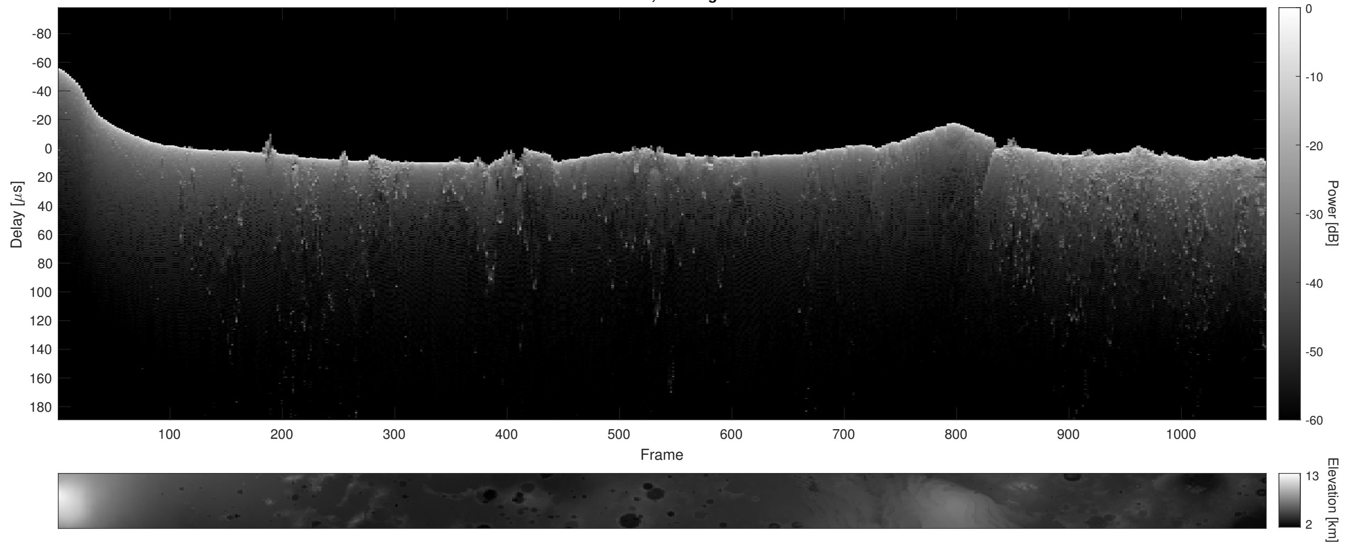
Orbit 2701, Cluttergram
