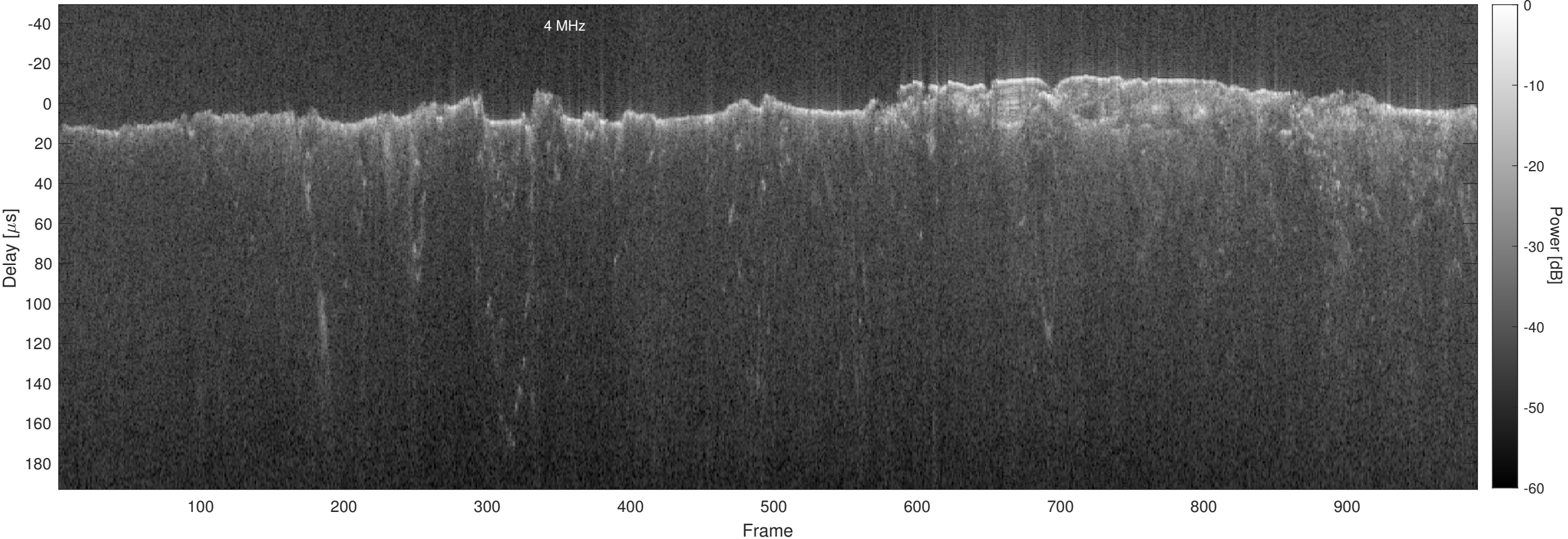
Orbit 2702, Optimized, No Window, Channel 2
