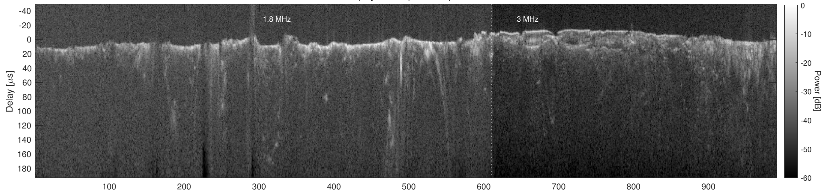
Orbit 2702, Cluttergram
