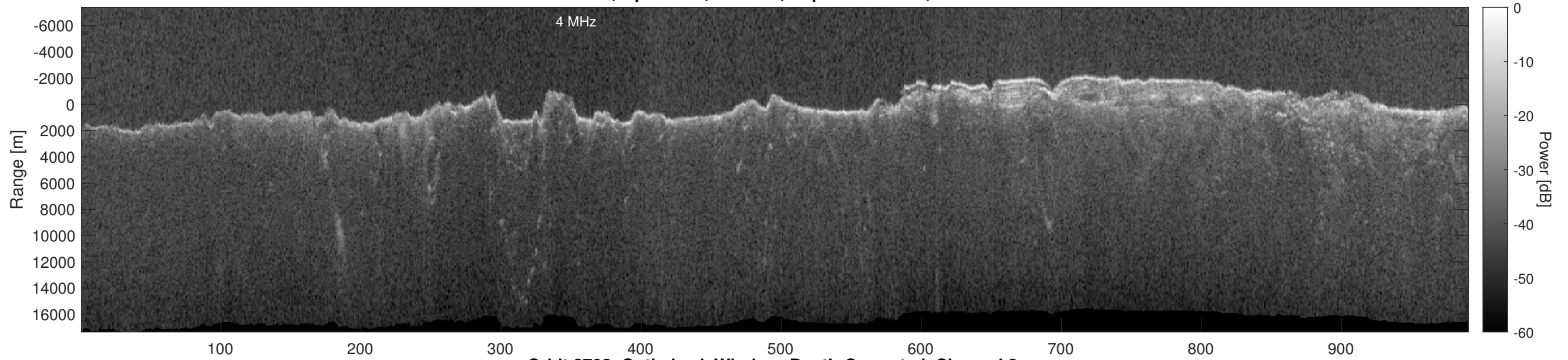
Orbit 2702, Optimized, Window, Depth-Corrected, Channel 2
