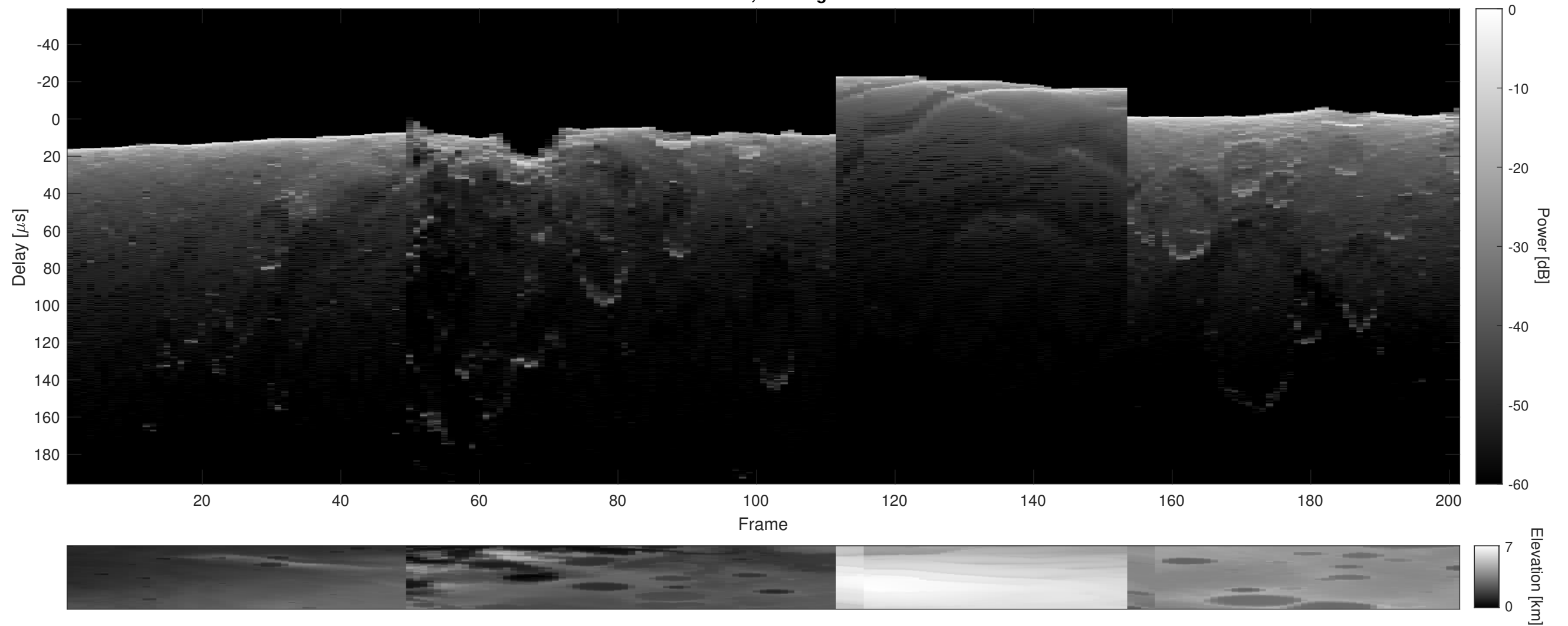
Orbit 2704, Cluttergram
